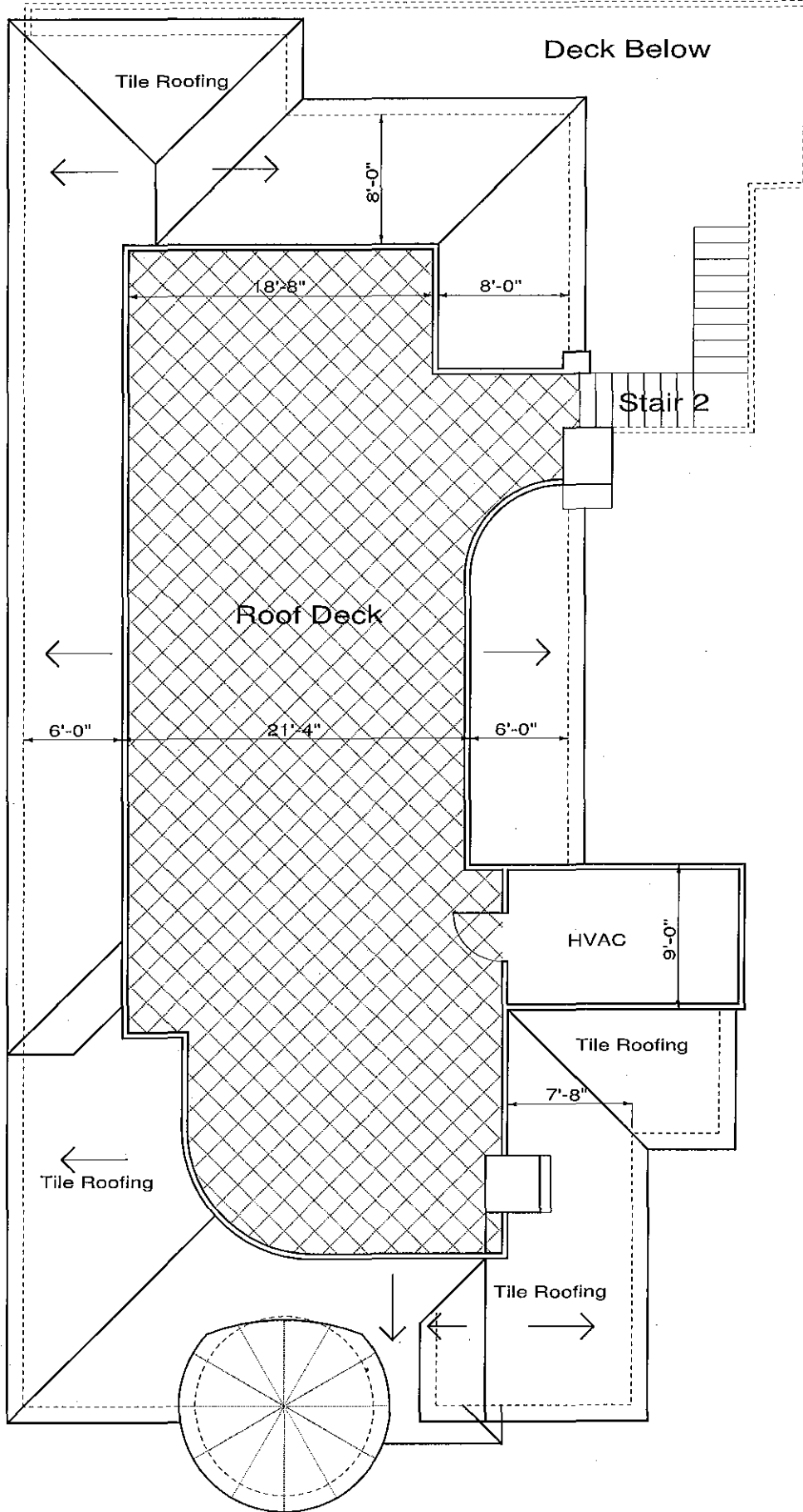
Roof Plan 1" = 8'
