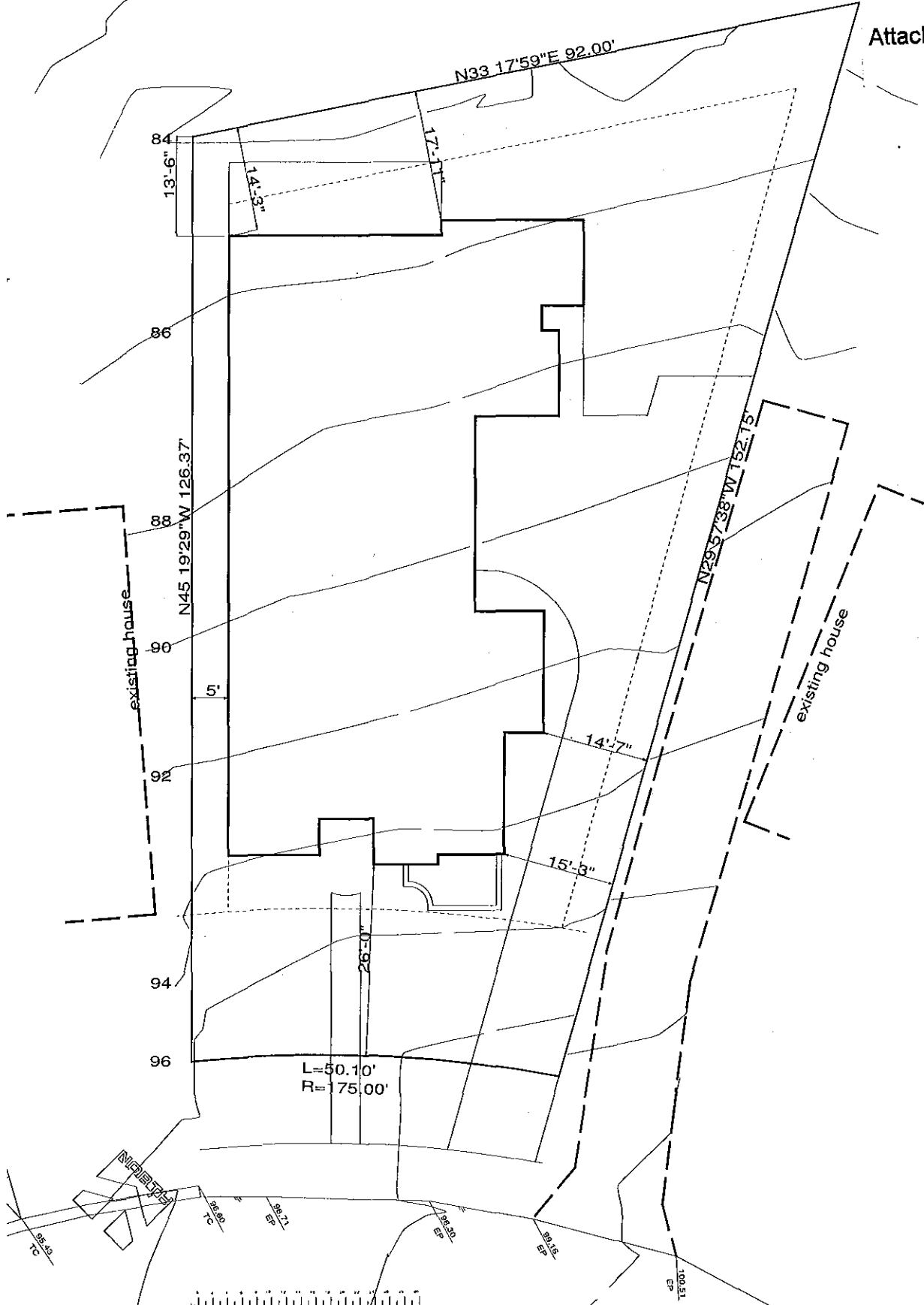
Site Plan 1" = 16' Third Street LOT 21 Block 4
